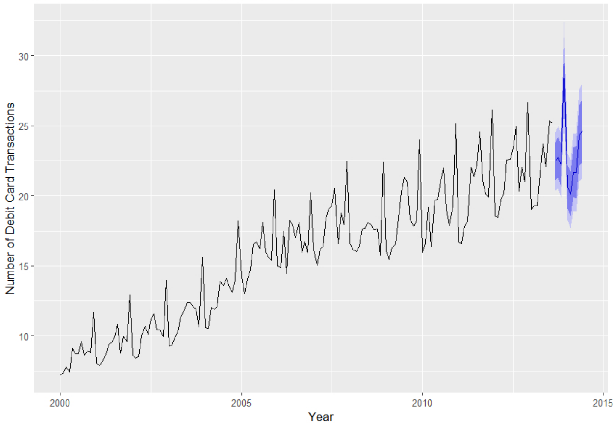
10-Step Ahead Forecast using ETS Model
