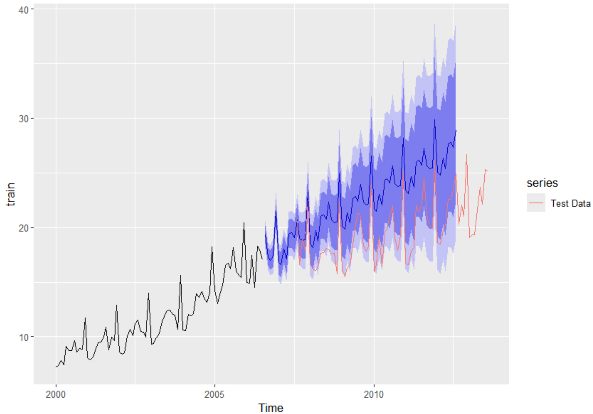
Forecasts from ARIMA(2,1,0)(0,1,1)[12]
