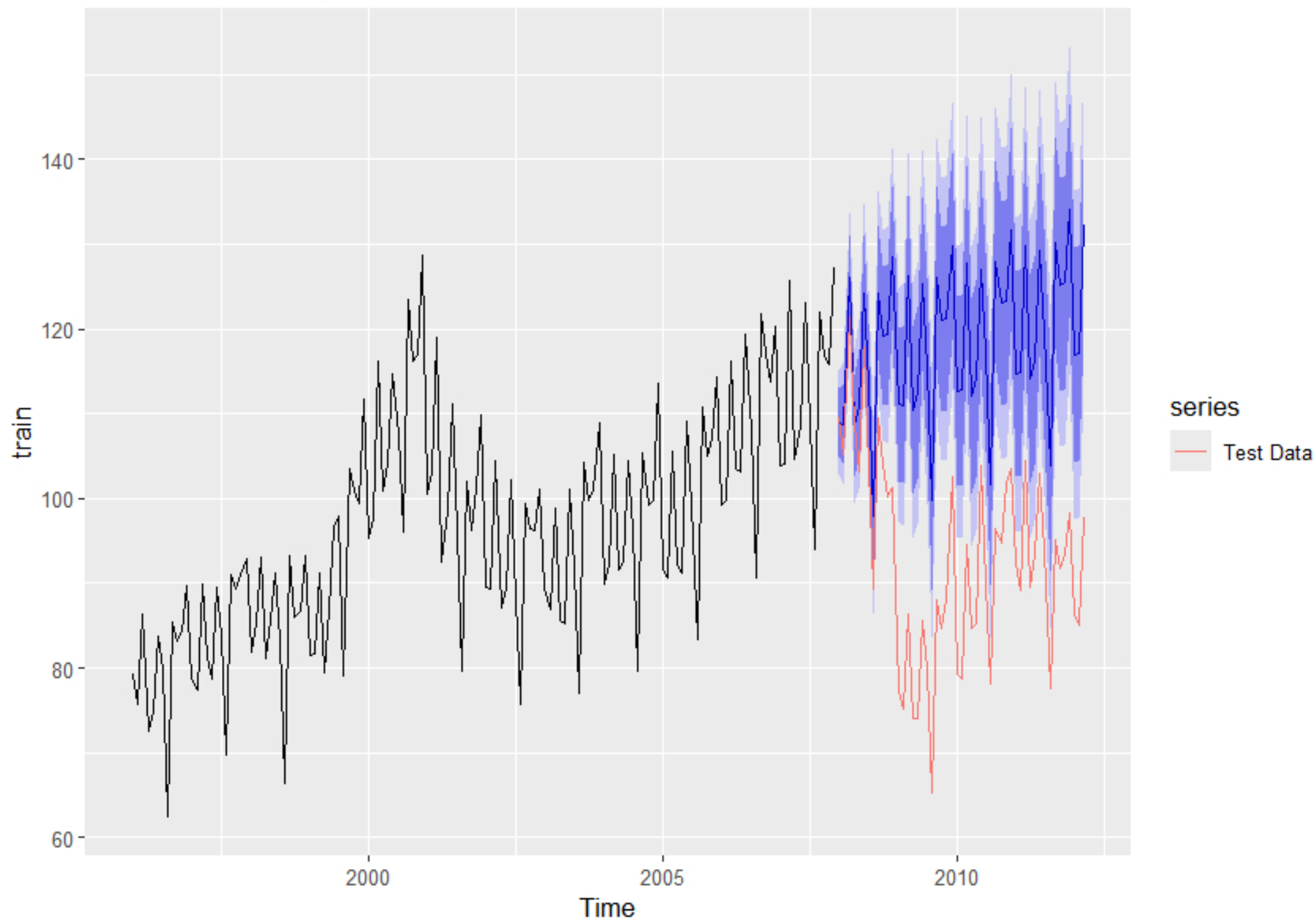
Forecasts from ARIMA(2,0,3)(0,1,2)[12] with drift
